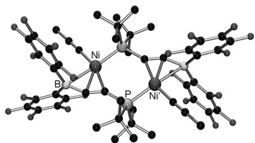
Figure 3. POV-ray drawing of 5 . All hydrogen atoms H are omitted for clarity. Selected bond lengths [Å] and angles [°]: Ni–C1 1.9536(12), Ni–C2 1.9714(13), Ni–B 2.3243(15), Ni–P 2.1982(4), Ni–N 1.8674(11), P–C(1) 1.7877(13), C2–B1 1.486(2), C1–C2 1.2681(18); C2–C1–P' 145.44(11), C1–C2–B 153.50(13).
